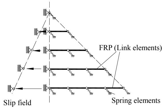
Figure 5 Simplified FE model for externally bonded FRP U-jackets on RC beam
