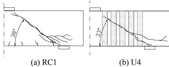
Figure 10 Diagonal cracks in RC1 and U4 at failure
