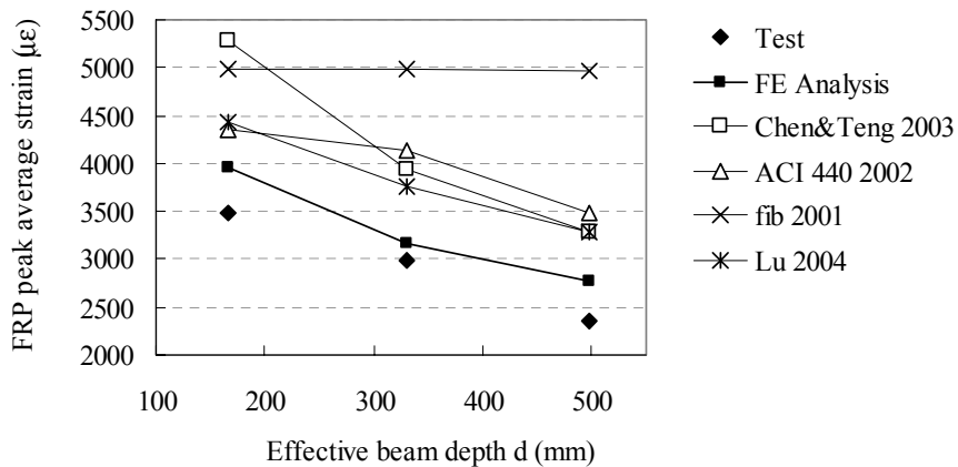
Figure 9 The peak average strains of FRP sheets
