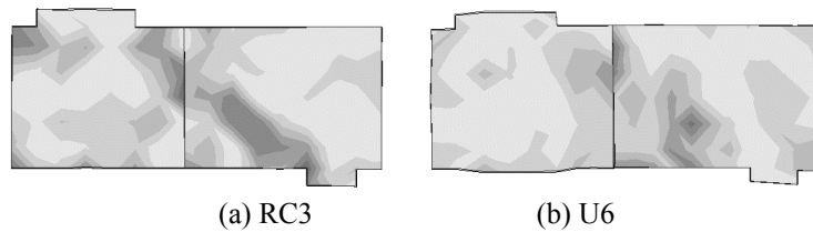
Figure 11 Principle tensile strain distributions on the webs of RC3 and U6 at a load of P \approx 0.75/P_u
