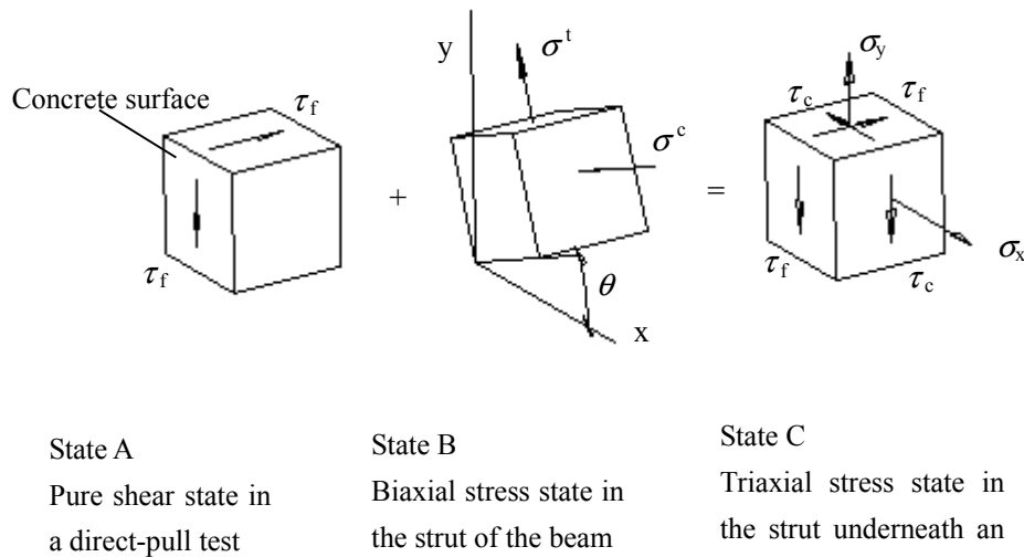
Figure 4 Superposition of stress states of concrete in the strut underneath the FRP sheets
