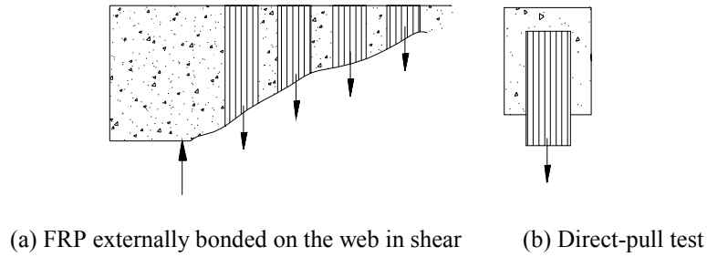
Figure 3 Loading condition of FRP sheets
