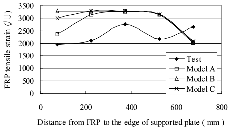
Figure 7 FRP strain distribution for different diagonal crack models: specimen U6
