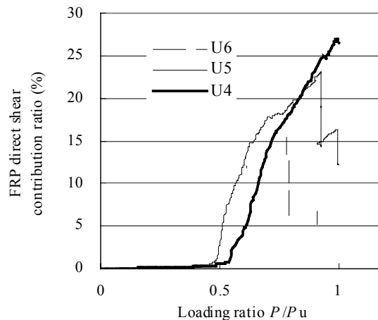
Figure 2 Development of the direct shear contribution of FRP sheets
