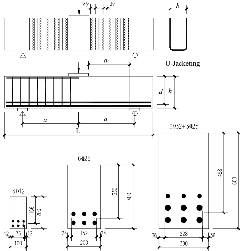
Figure 2 Configurations of specimens
