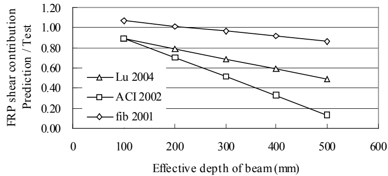
Figure 1 Size effect on shear contribution of FRP sheets
