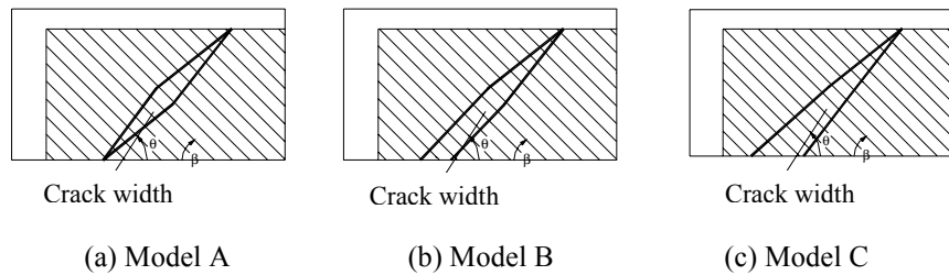
Figure 6 Simplified diagonal crack models by Lu et al. (2005a)
