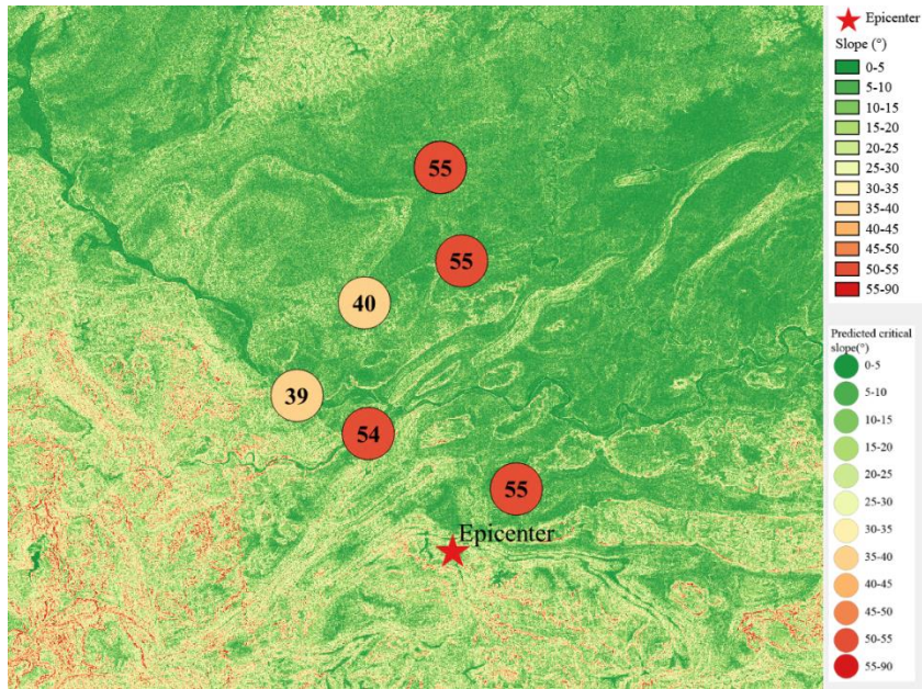
(a) The proportion of the landslide slab thickness that is saturated equals 0%
