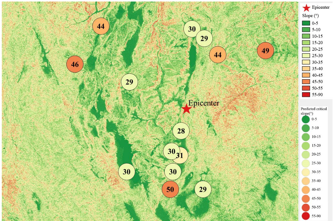
(c) The proportion of the landslide slab thickness that is saturated equals 90% Figure 4 Distribution of earthquake-induced landslide near to different stations
