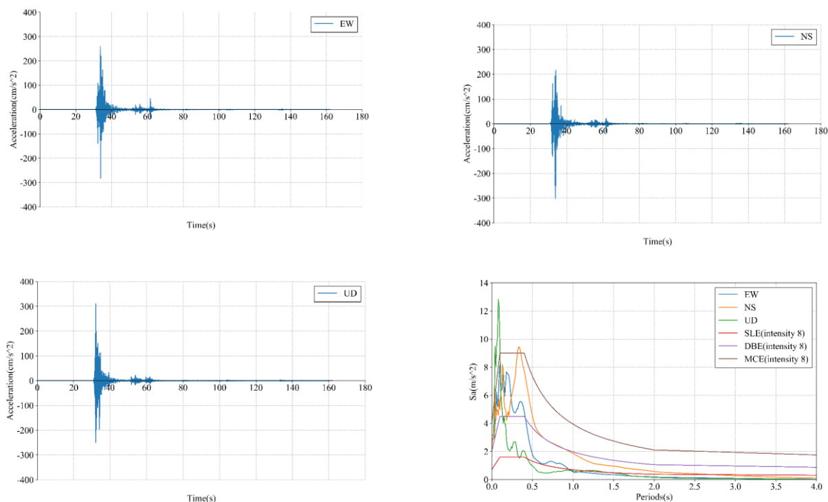
Figure 1 Waveform and response spectra of the recorded ground motions with maximal PGA
