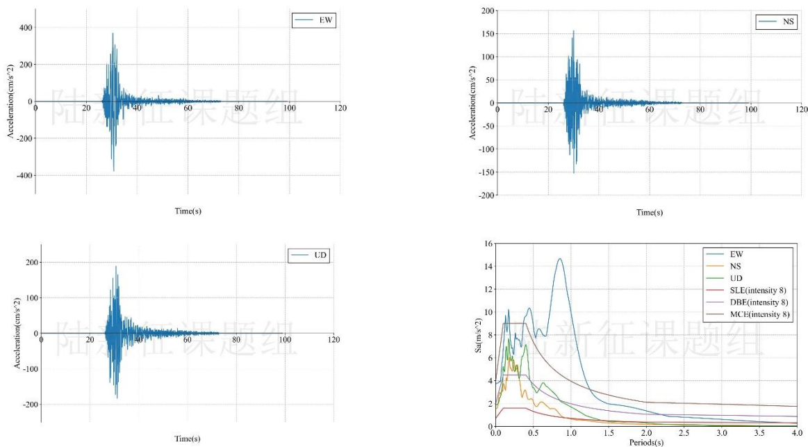
Figure 1 Typical waveform and response spectra of the recorded ground motions
